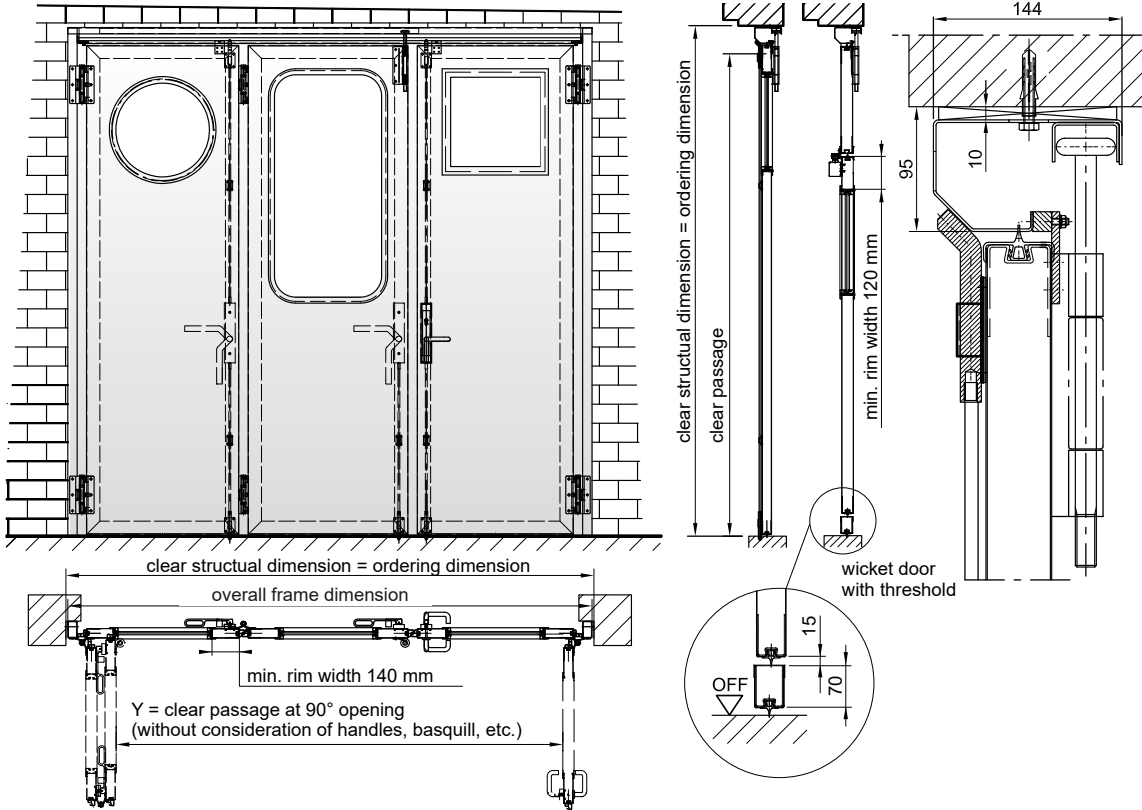
Installation in front of the soffit (90° outward opening shown)
