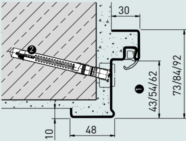
Corner frame for 62er doors, wall plug assembly
