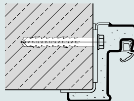
Weld installation with sliding anchor (exposed masonry)
