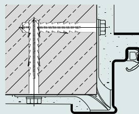
Wall anchor, dowelled, (masonry/concrete)
