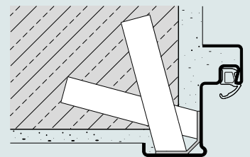
Wall anchor, mortared, (masonry/concrete)
