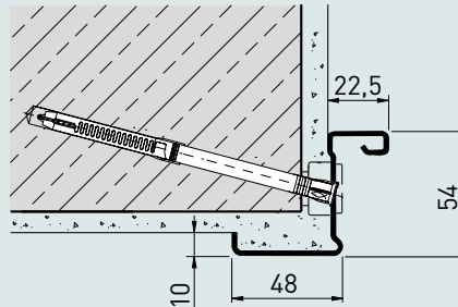
Corner frame for 42 mm doors, wall plug assembly (masonry/concrete)
