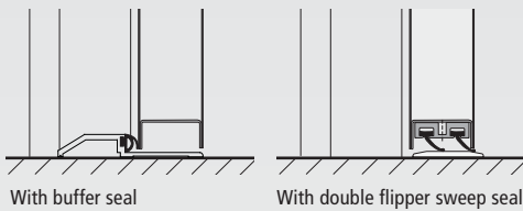
Optional floor seal
