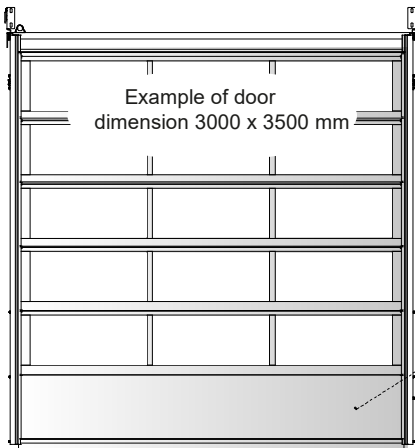
SLW 40 (exterior view) Bottom section 625 mm Normal-fitting N
