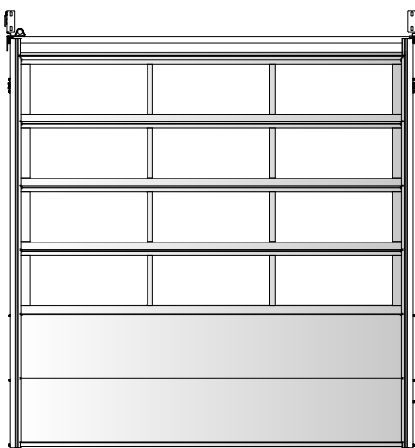
SLW 40 (exterior view) Bottom section 1250 mm Normal-fitting N
