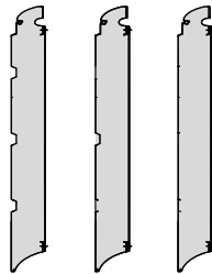
SLW 40 (exterior view) Bottom section 1250 mm Normal-fitting N
