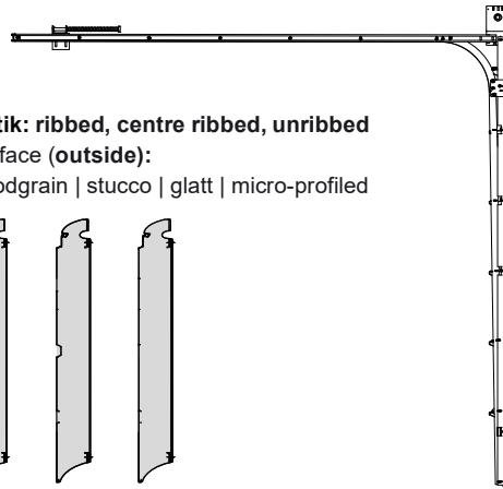
SLW 40 (exterior view) Bottom section 625 mm Normal-fitting N
